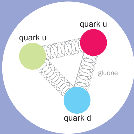
protone
