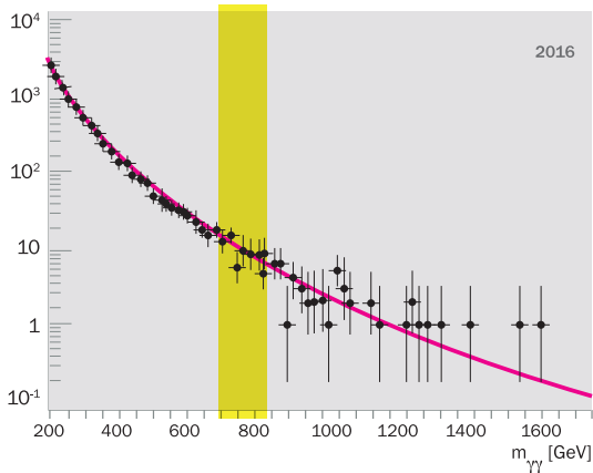
ATLAS event/20 GeV
