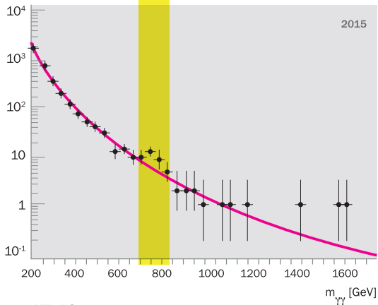
ATLAS event/20 GeV
