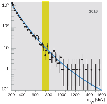
CMS event/20 GeV
